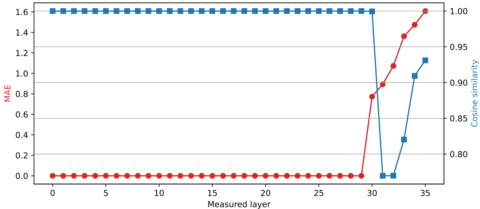
Qwen2.5-3B | Quantized layer 29 | float64 \rightarrow int2
