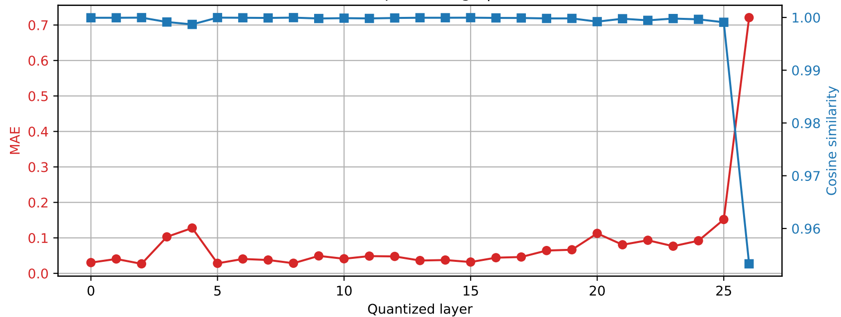
Qwen2.5-7B-Instruct | Prompt 0 Final RMSNorm output damage | float16 \rightarrow int8
