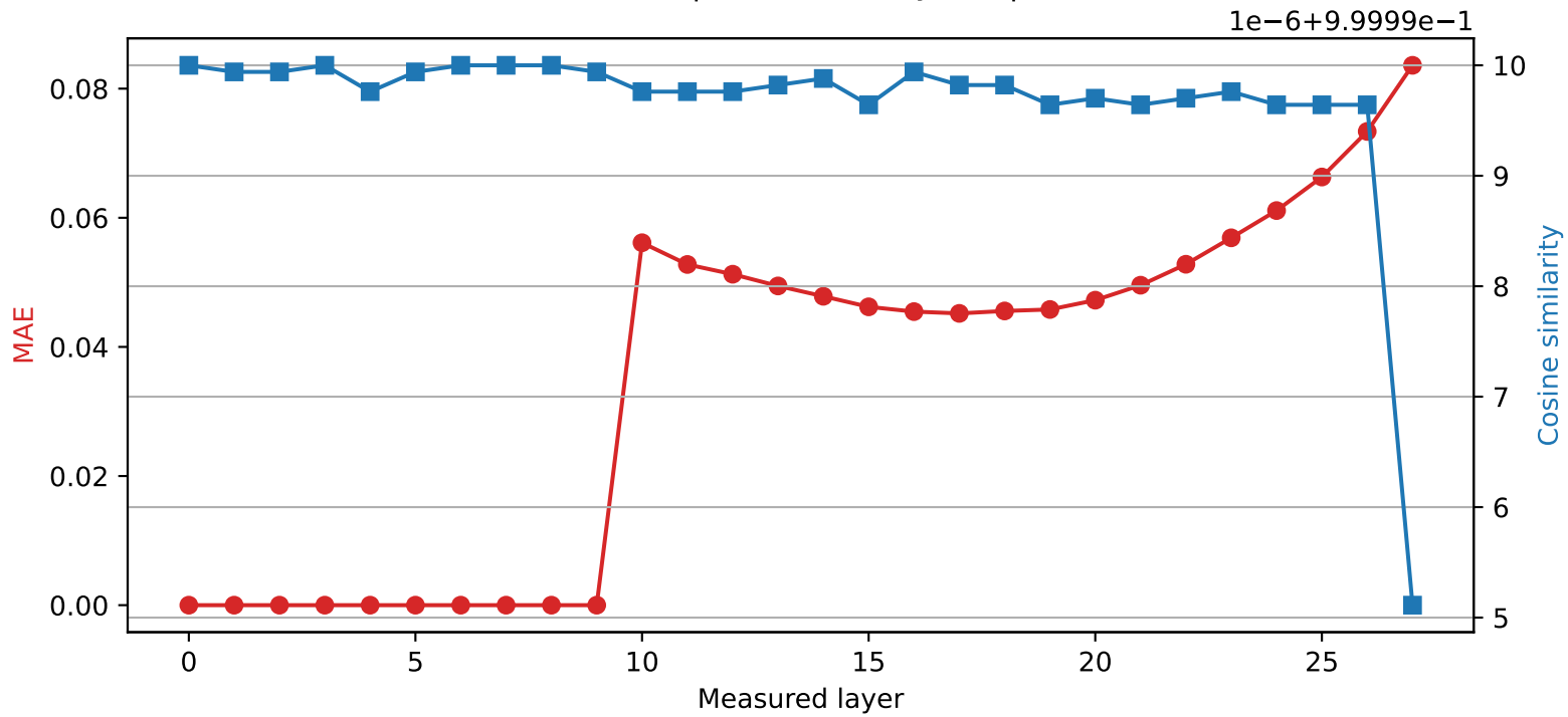
Qwen2.5-7B-Instruct | Quantized layer 9 | float16 \rightarrow int8
