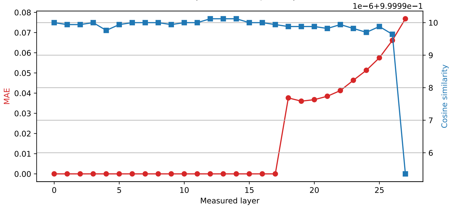
Qwen2.5-7B-Instruct | Quantized layer 17 | float16 → int8
