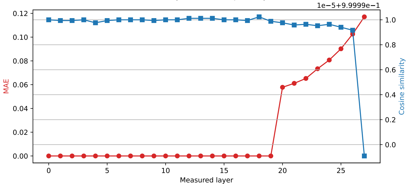
Qwen2.5-7B-Instruct | Quantized layer 19 | float16 → int8
