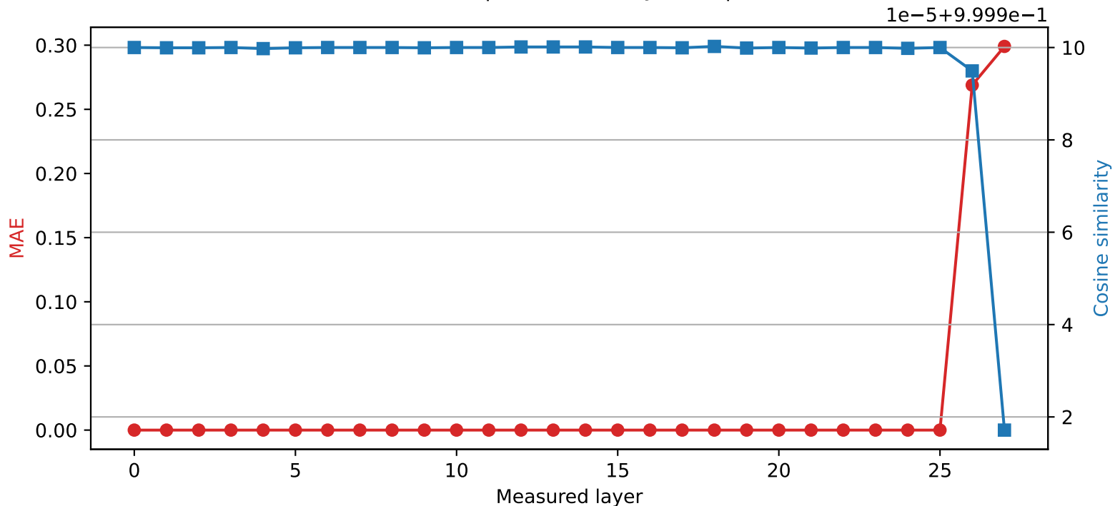
Qwen2.5-7B-Instruct | Quantized layer 25 | float16 \rightarrow int8
