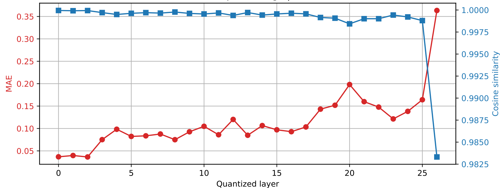
Qwen2.5-7B-Instruct | Prompt 1 Final RMSNorm output damage | float16 \rightarrow int8
