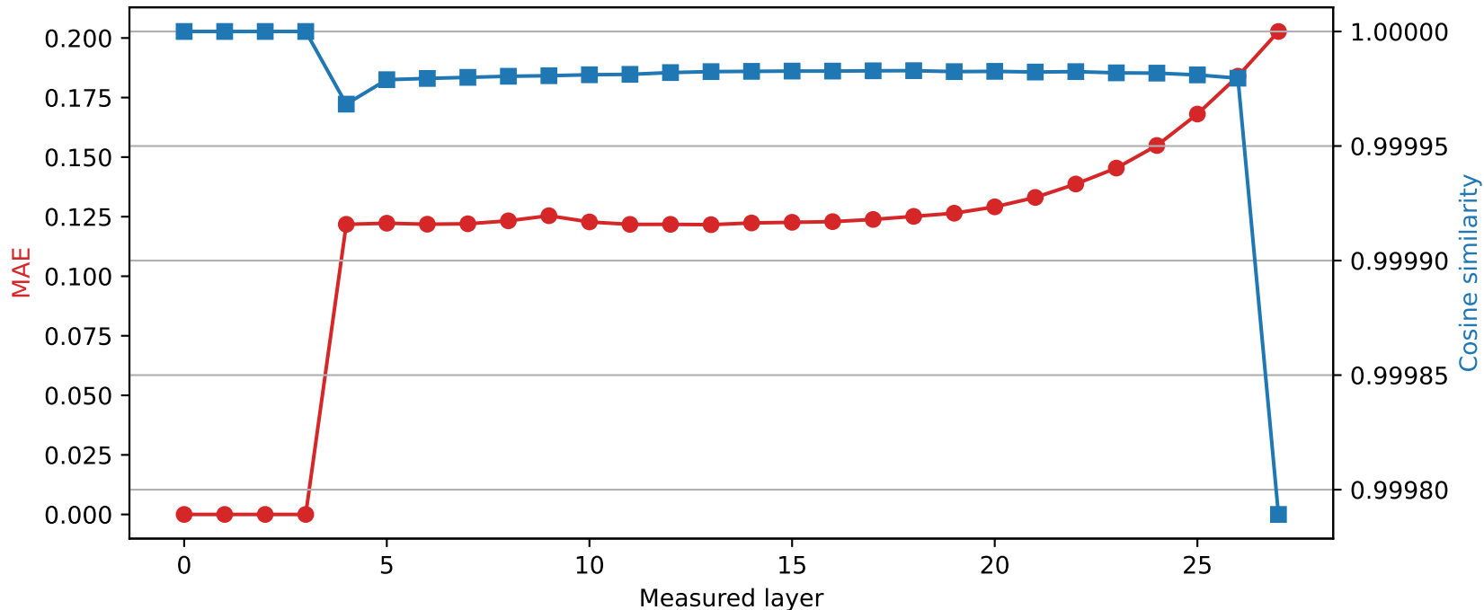
Qwen2.5-7B-Instruct | Quantized layer 3 | float16 \rightarrow int8
