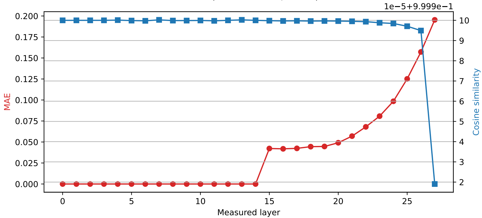
Qwen2.5-7B-Instruct | Quantized layer 14 | float16 \rightarrow int8
