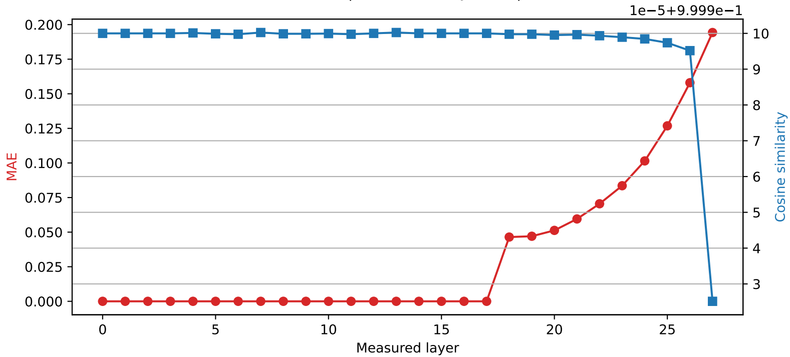
Qwen2.5-7B-Instruct | Quantized layer 17 | float16 \rightarrow int8
