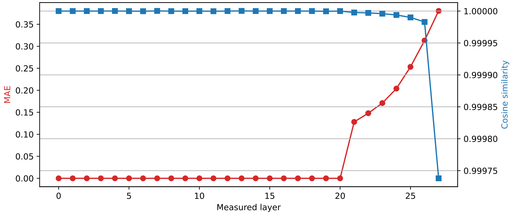
Qwen2.5-7B-Instruct | Quantized layer 20 | float16 \rightarrow int8
