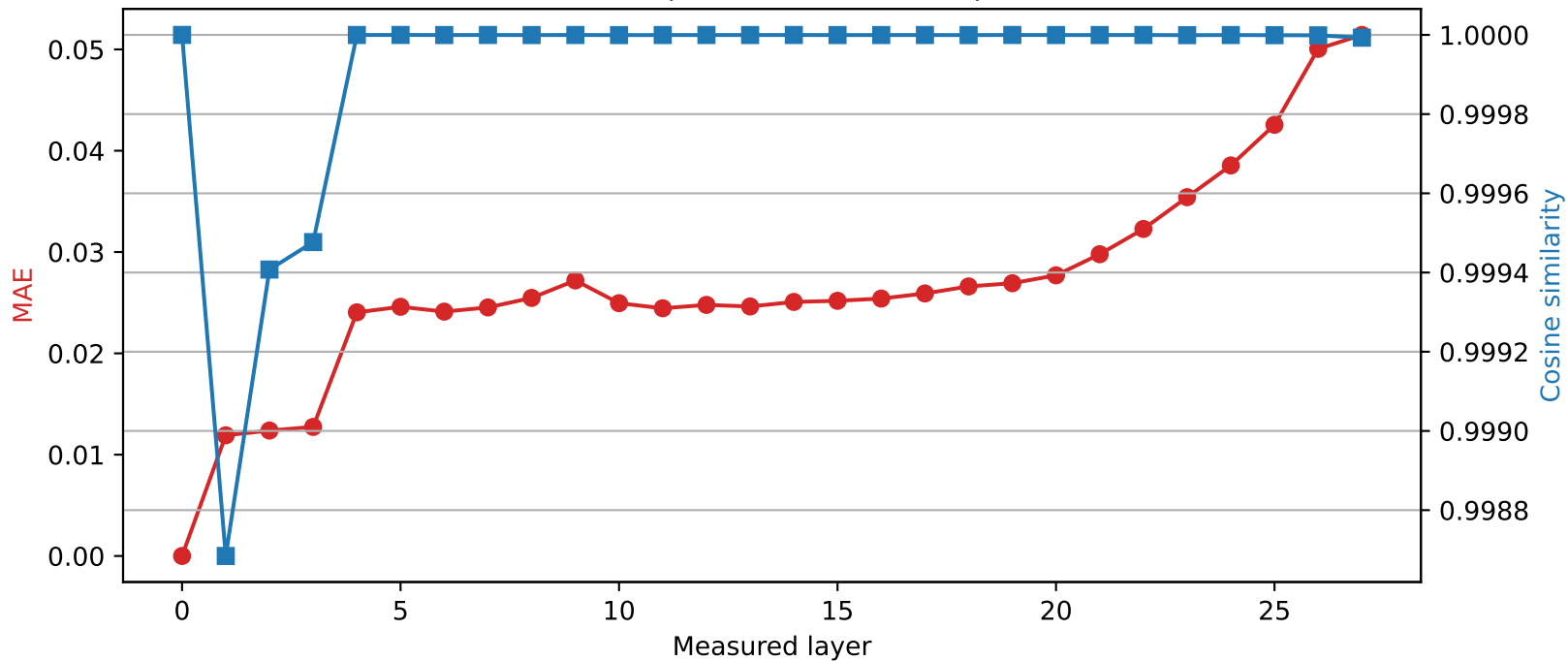
Qwen2.5-7B-Instruct | Quantized layer 0 | float16 \rightarrow int8
