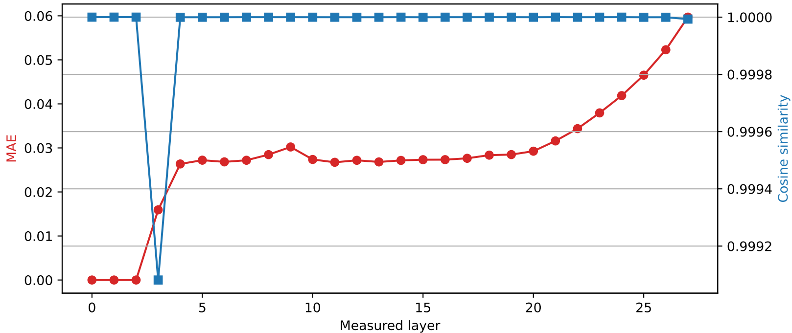
Qwen2.5-7B-Instruct | Quantized layer 2 | float16 → int8
