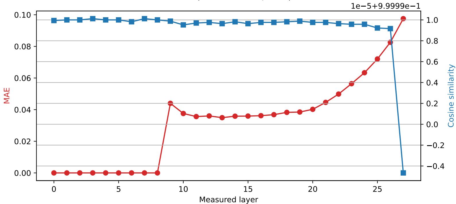
Qwen2.5-7B-Instruct | Quantized layer 8 | float16 → int8
