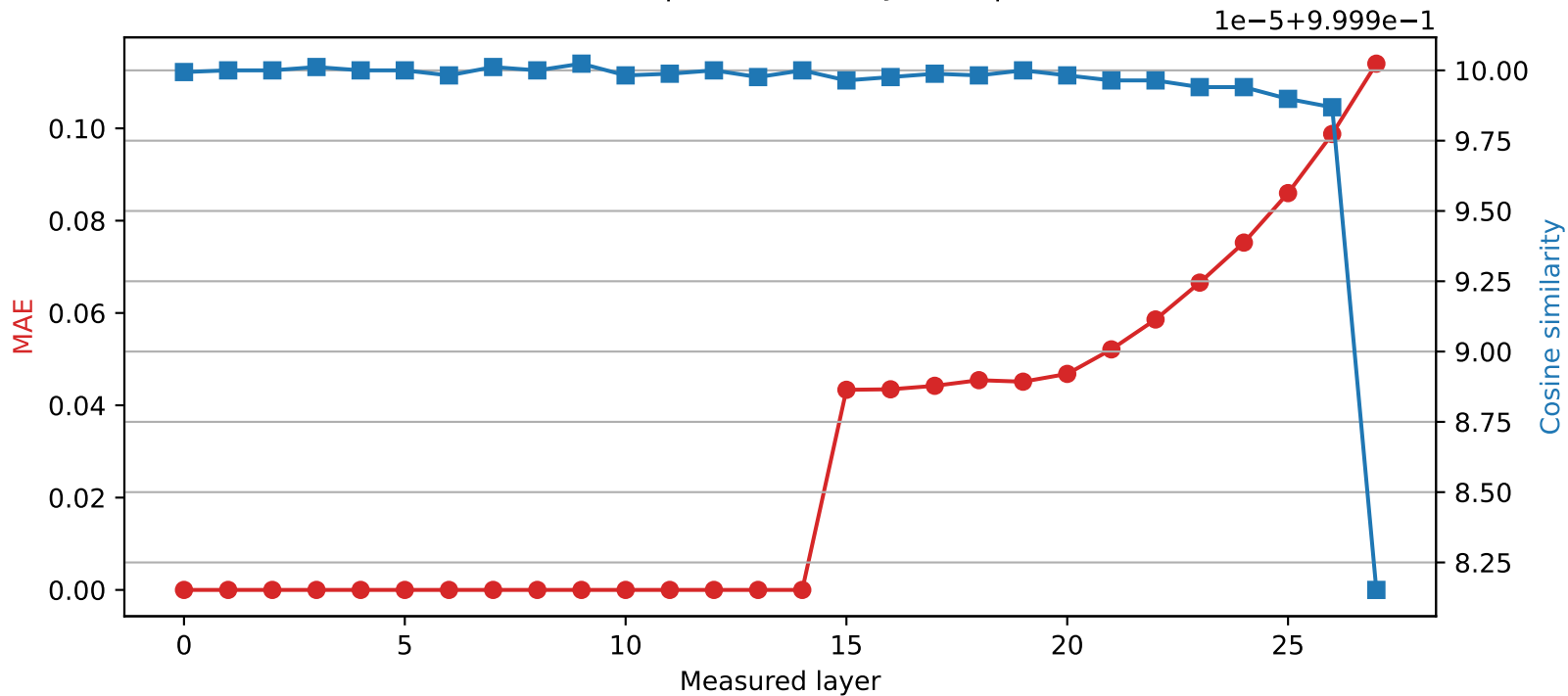
Qwen2.5-7B-Instruct | Quantized layer 14 | float16 → int8
