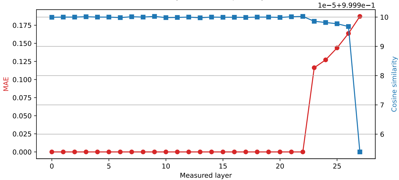
Qwen2.5-7B-Instruct | Quantized layer 22 | float16 \rightarrow int8
