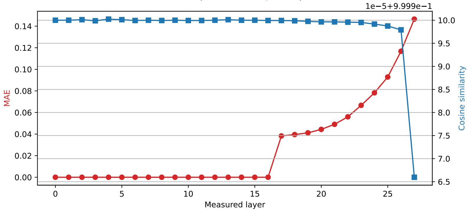
Qwen2.5-7B-Instruct | Quantized layer 16 | float16 \rightarrow int8
