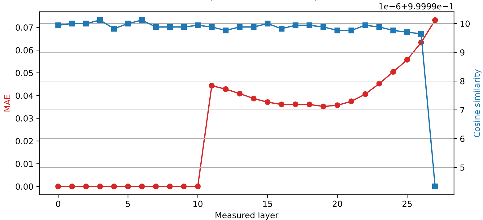
Qwen2.5-7B-Instruct | Quantized layer 10 | float16 → int8
