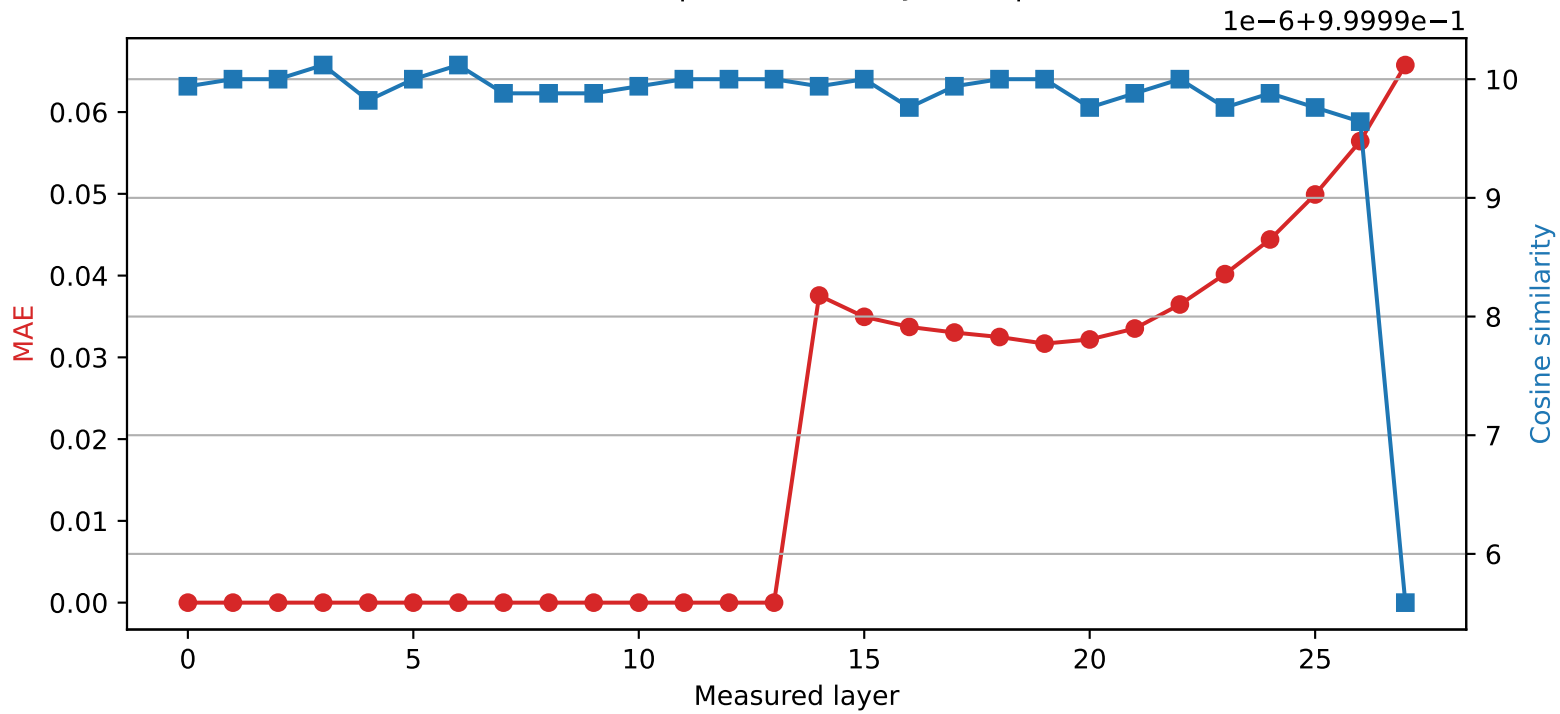
Qwen2.5-7B-Instruct | Quantized layer 13 | float16 \rightarrow int8
