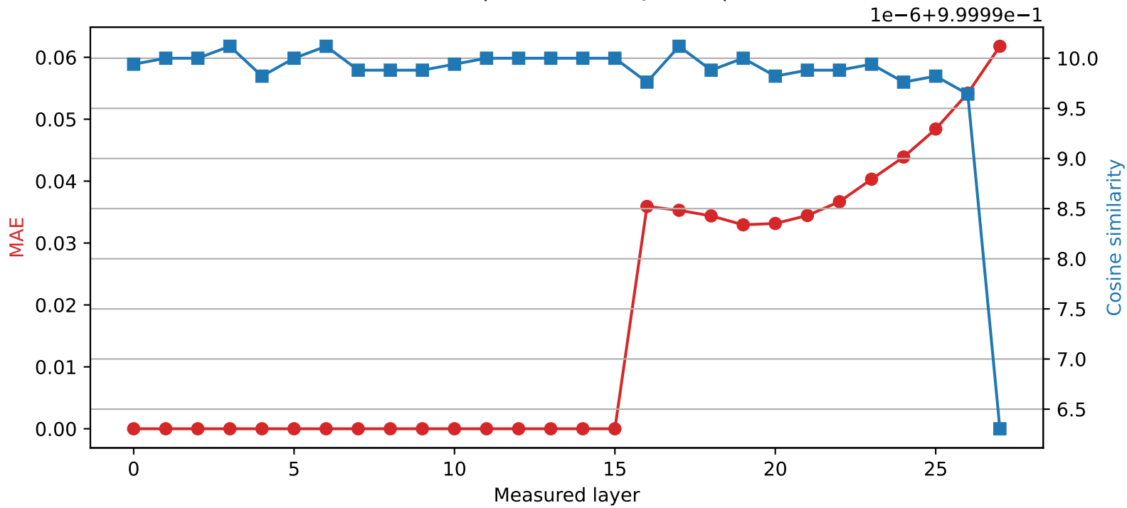
Qwen2.5-7B-Instruct | Quantized layer 15 | float16 → int8
