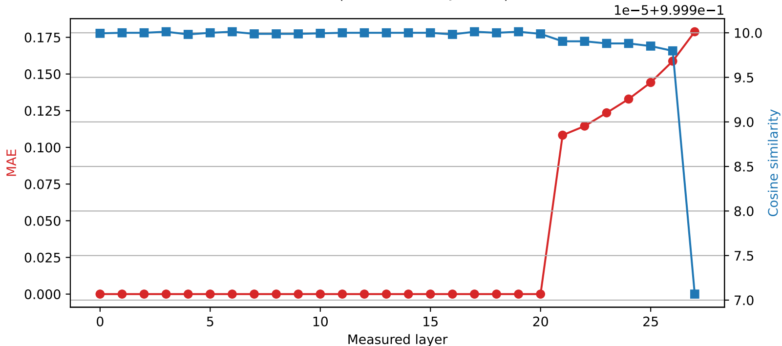
Qwen2.5-7B-Instruct | Quantized layer 20 | float16 → int8
