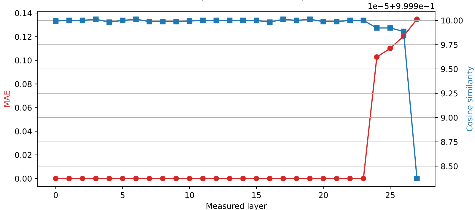
Qwen2.5-7B-Instruct | Quantized layer 23 | float16 \rightarrow int8
