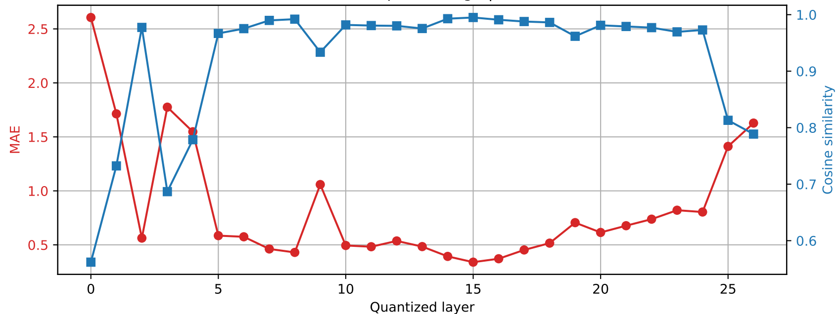
Qwen2.5-7B-Instruct | Prompt 0 Final RMSNorm output damage | float16 \rightarrow int4
