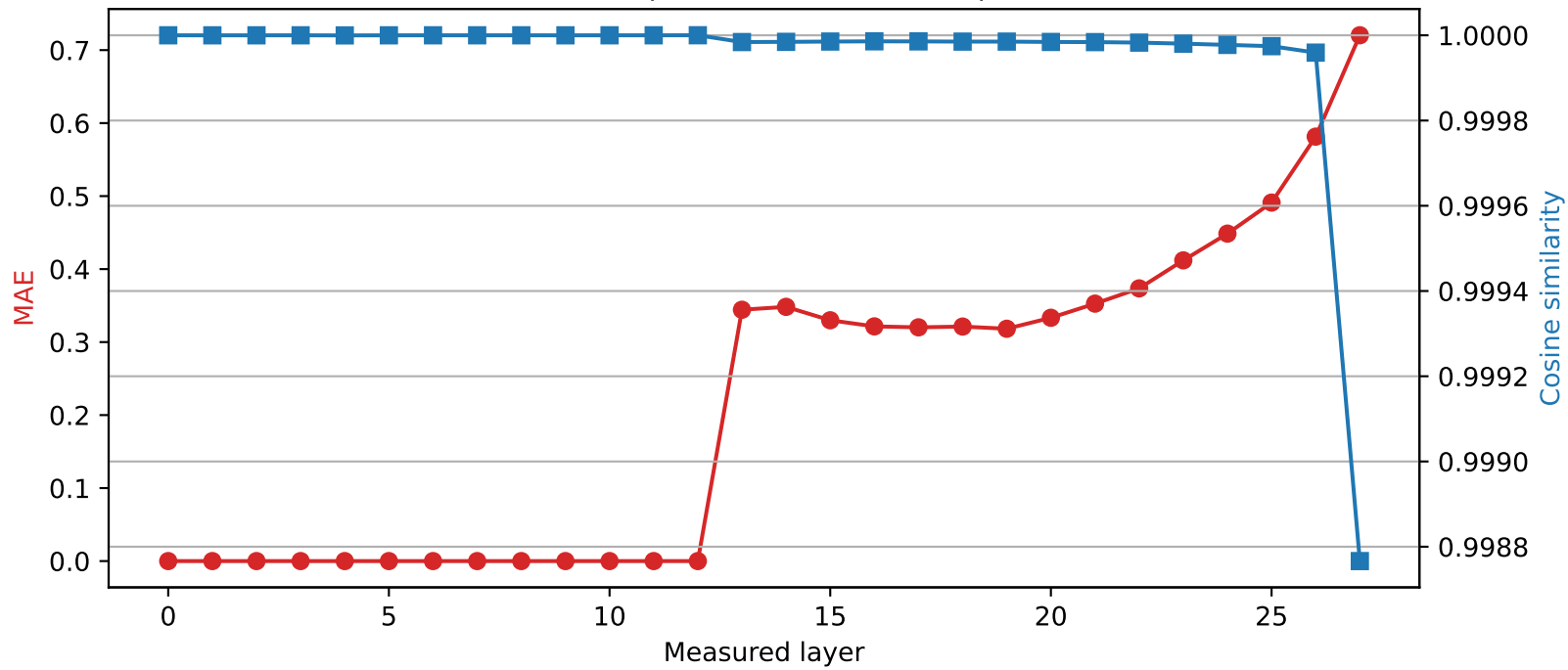
Qwen2.5-7B-Instruct | Quantized layer 12 | float16 \rightarrow int4
