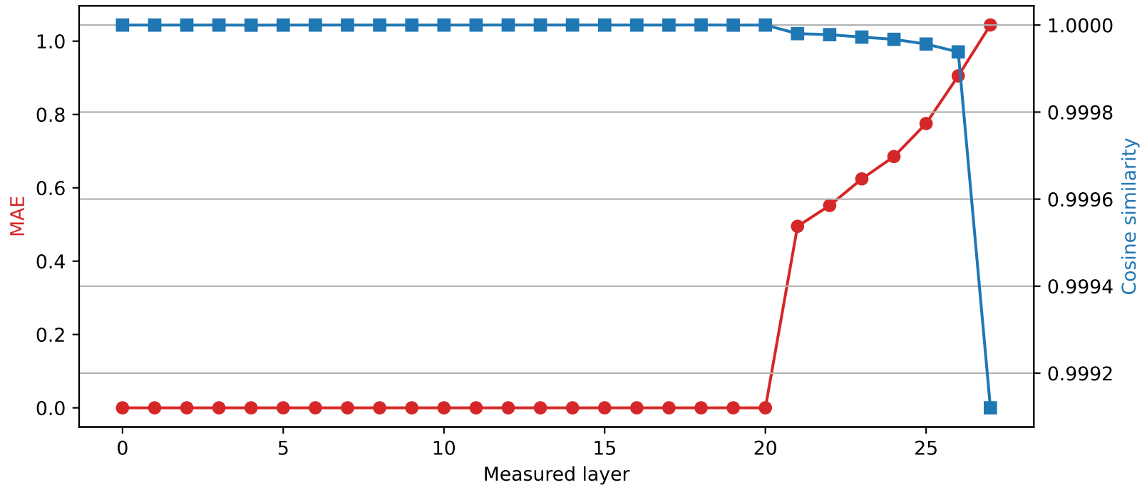
Qwen2.5-7B-Instruct | Quantized layer 20 | float16 \rightarrow int4
