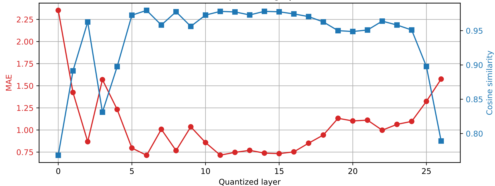
Qwen2.5-7B-Instruct | Prompt 1 Final RMSNorm output damage | float16 \rightarrow int4
