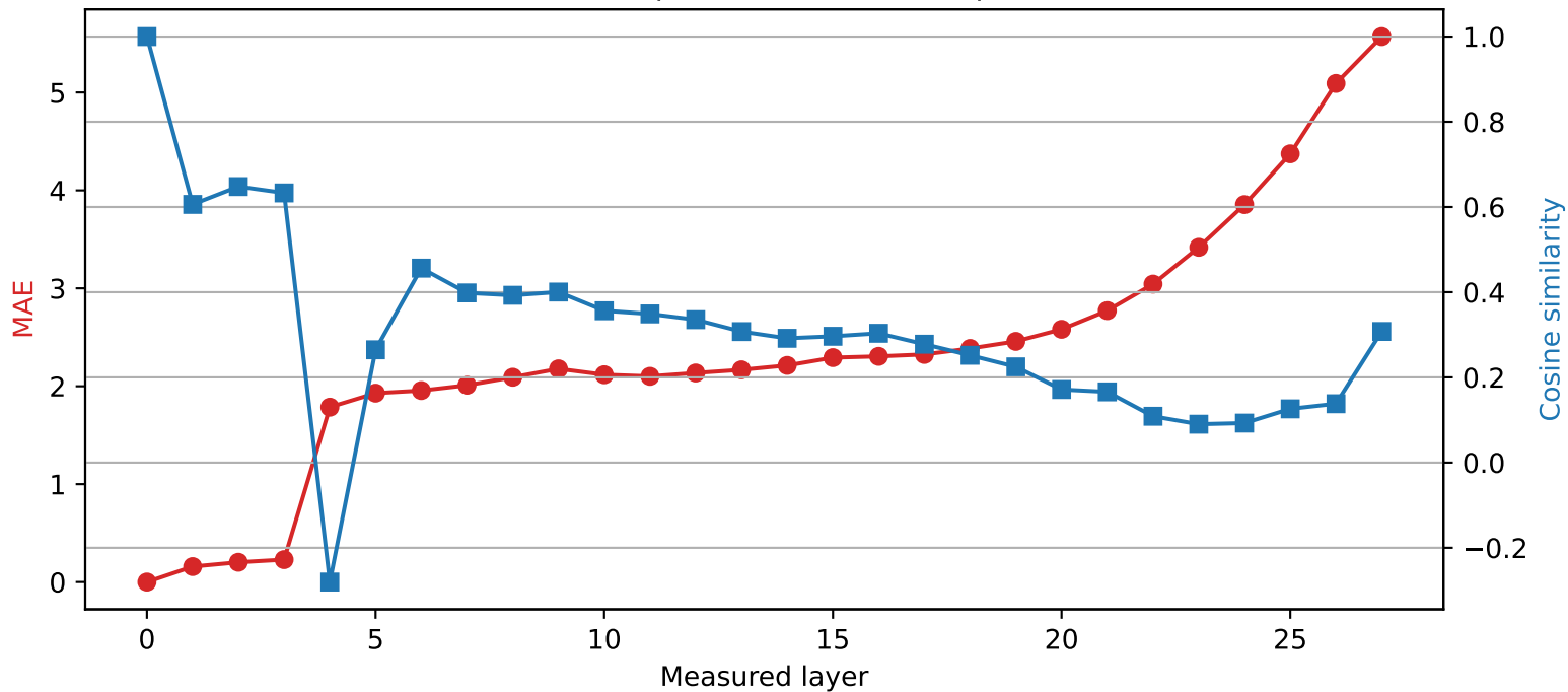
Qwen2.5-7B-Instruct | Quantized layer 0 | float16 \rightarrow int4
