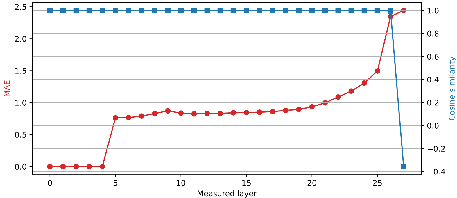
Qwen2.5-7B-Instruct | Quantized layer 4 | float16 \rightarrow int4
