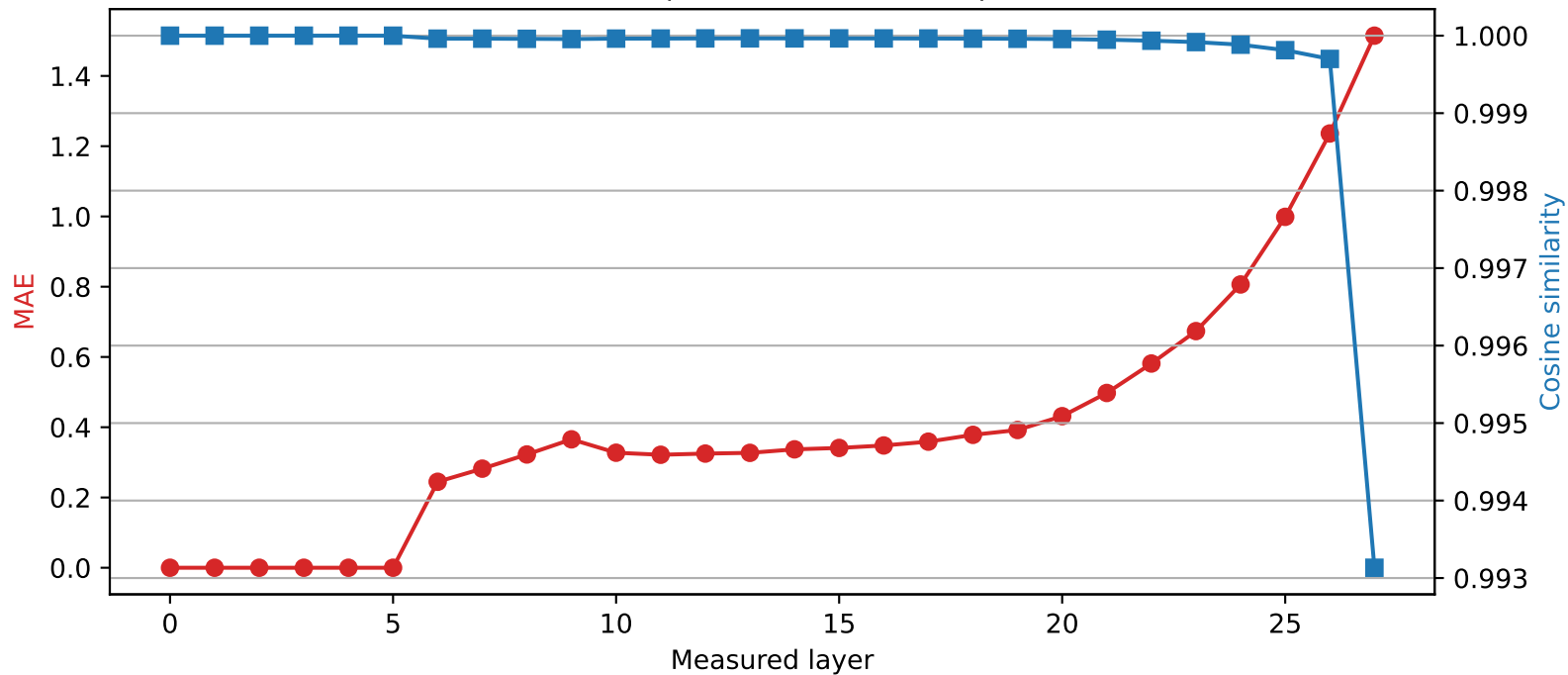
Qwen2.5-7B-Instruct | Quantized layer 5 | float16 → int4
