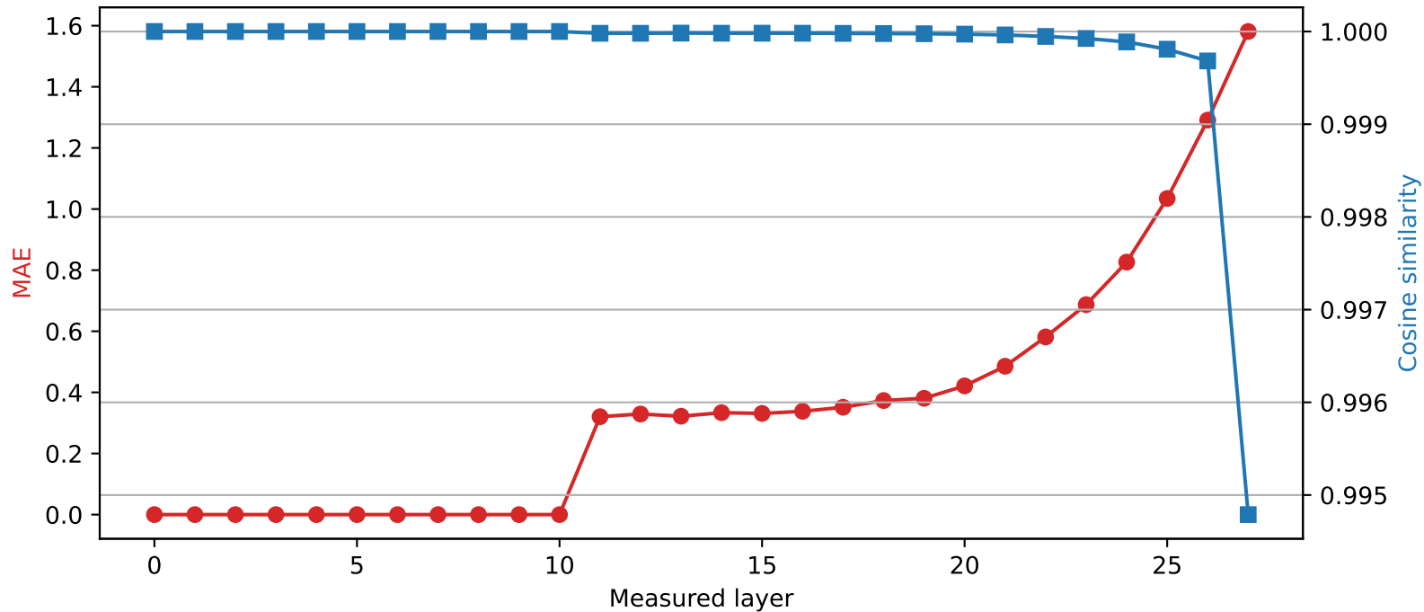
Qwen2.5-7B-Instruct | Quantized layer 10 | float16 \rightarrow int4
