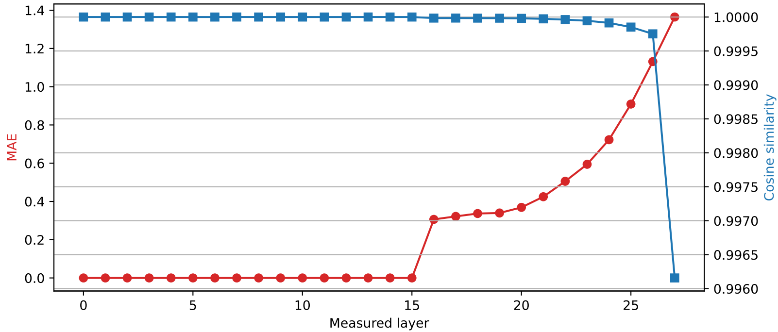
Qwen2.5-7B-Instruct | Quantized layer 15 | float16 \rightarrow int4
