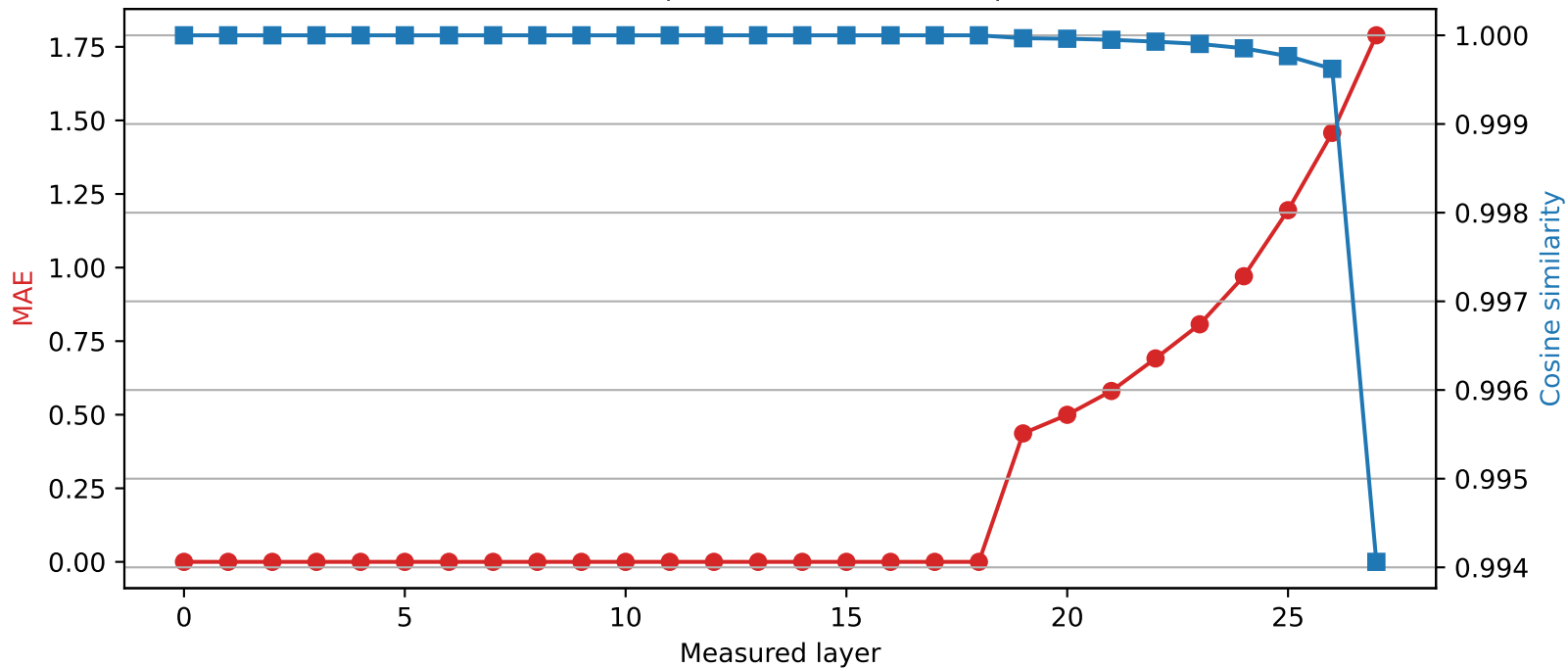
Qwen2.5-7B-Instruct | Quantized layer 18 | float16 \rightarrow int4
