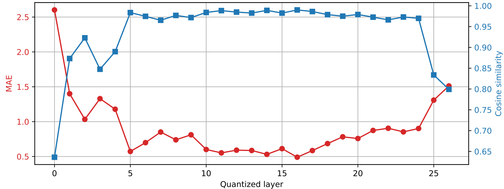
Qwen2.5-7B-Instruct | Prompt 2 Final RMSNorm output damage | float16 \rightarrow int4
