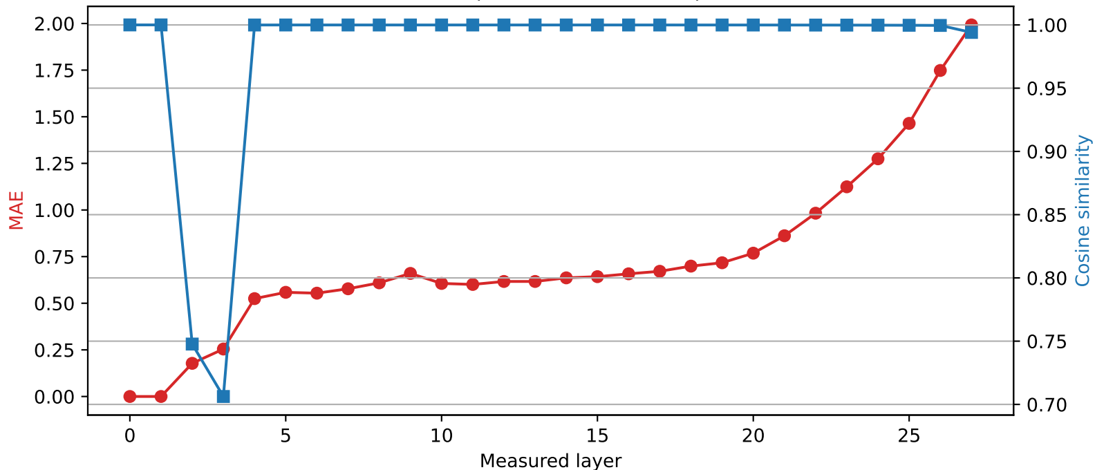
Qwen2.5-7B-Instruct | Quantized layer 1 | float16 → int4
