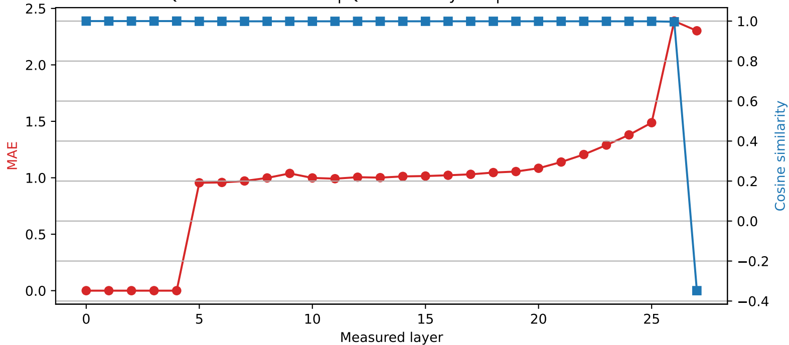
Qwen2.5-7B-Instruct | Quantized layer 4 | float16 → int4
