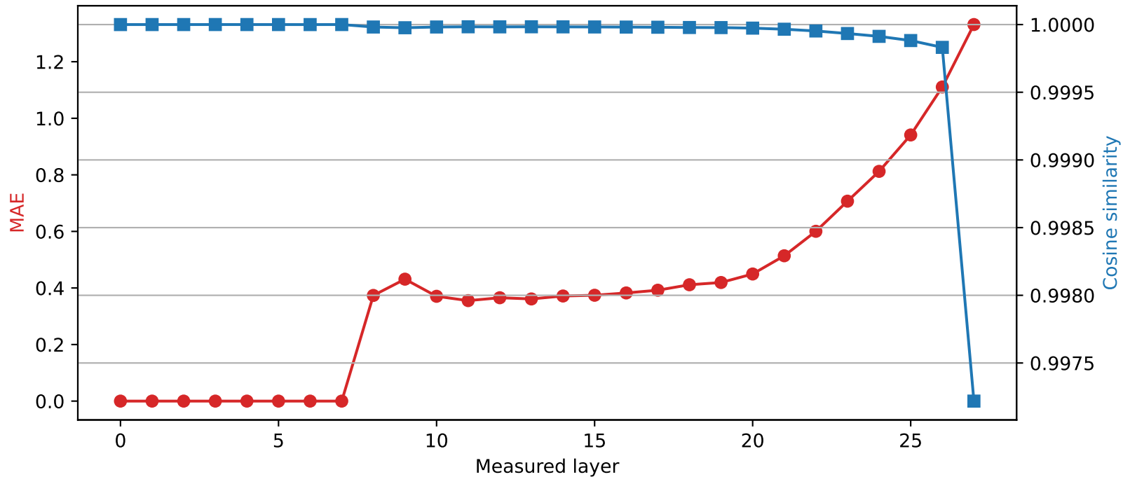
Qwen2.5-7B-Instruct | Quantized layer 7 | float16 \rightarrow int4
