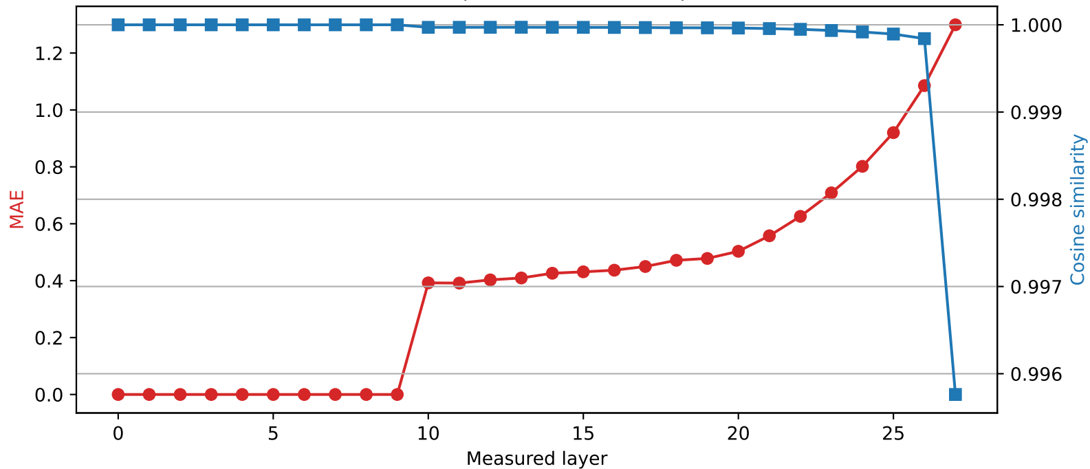
Qwen2.5-7B-Instruct | Quantized layer 9 | float16 → int4
