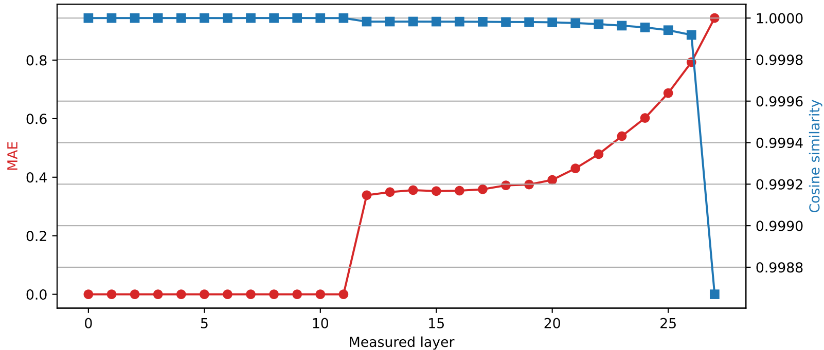
Qwen2.5-7B-Instruct | Quantized layer 11 | float16 → int4
