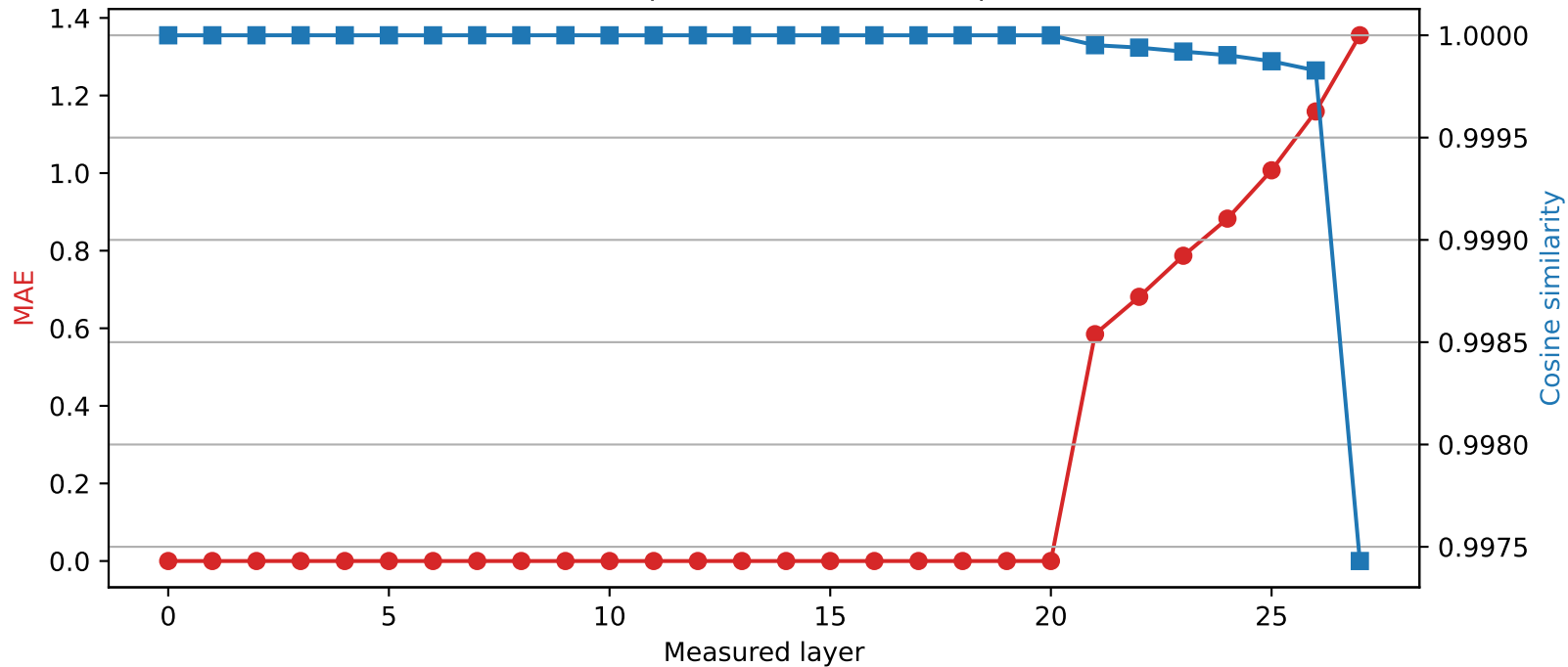
Qwen2.5-7B-Instruct | Quantized layer 20 | float16 → int4
