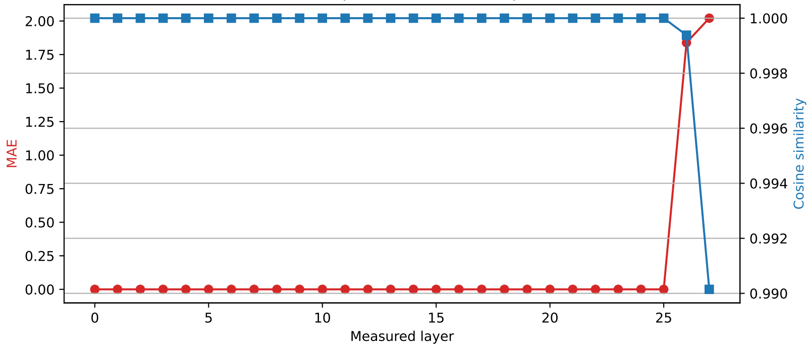
Qwen2.5-7B-Instruct | Quantized layer 25 | float16 → int4
