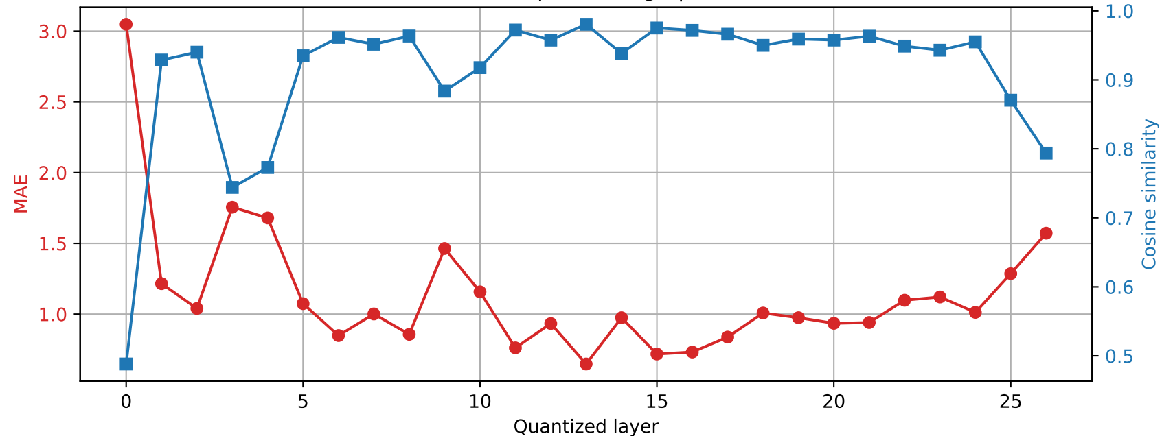
Qwen2.5-7B-Instruct | Prompt 3 Final RMSNorm output damage | float16 \rightarrow int4
