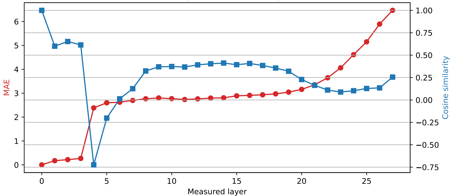
Qwen2.5-7B-Instruct | Quantized layer 0 | float16 → int4
