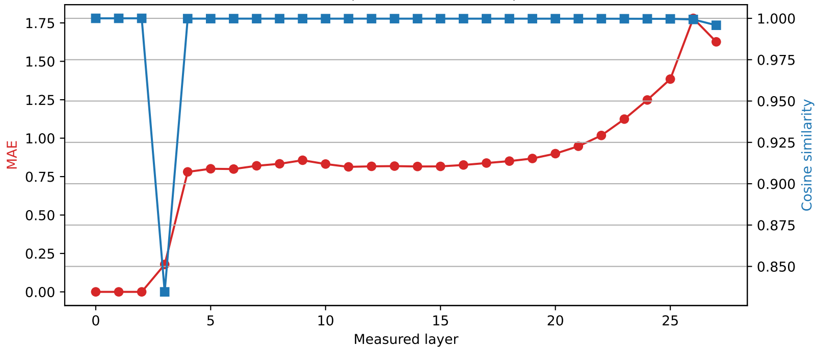
Qwen2.5-7B-Instruct | Quantized layer 2 | float16 \rightarrow int4
