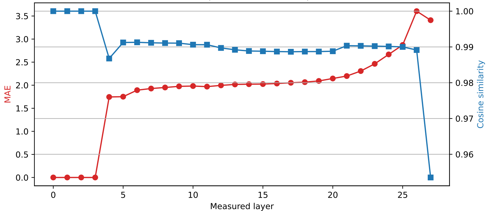
Qwen2.5-7B-Instruct | Quantized layer 3 | float16 \rightarrow int4
