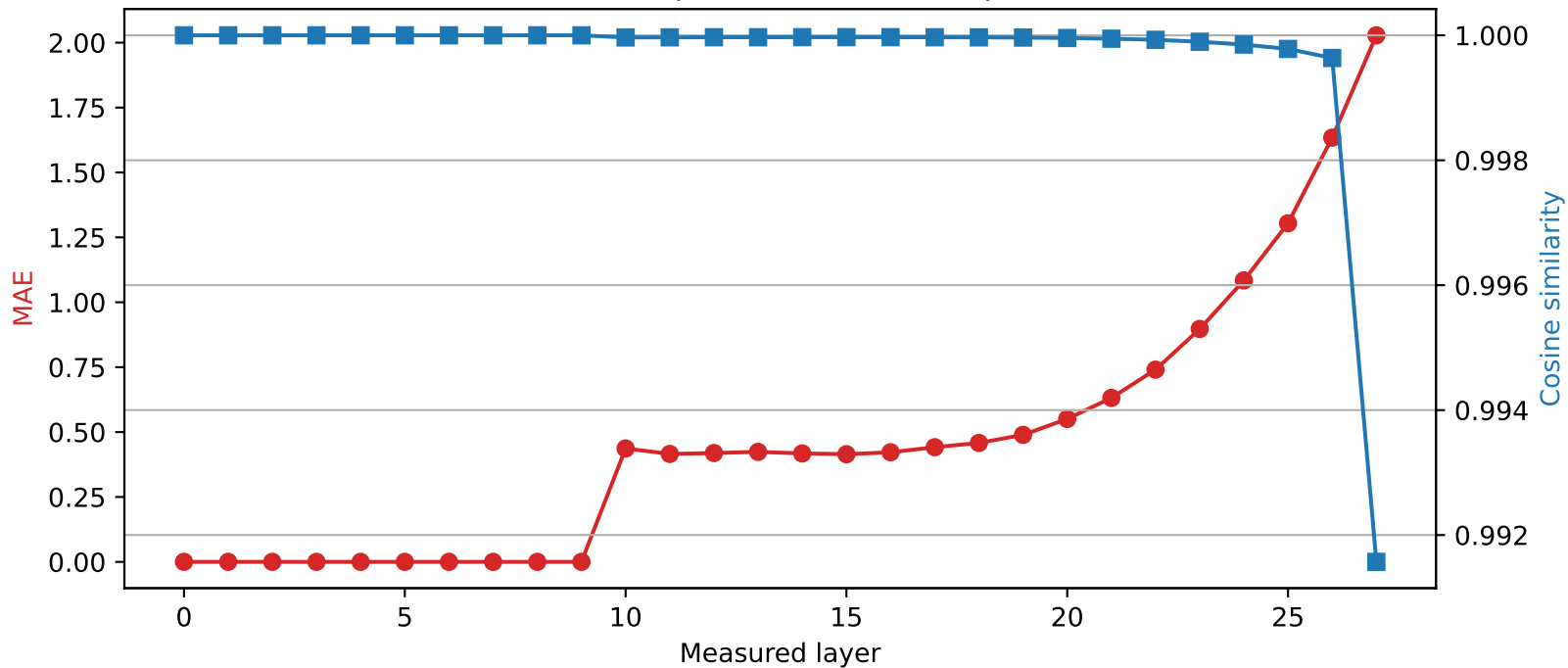
Qwen2.5-7B-Instruct | Quantized layer 9 | float16 \rightarrow int4
