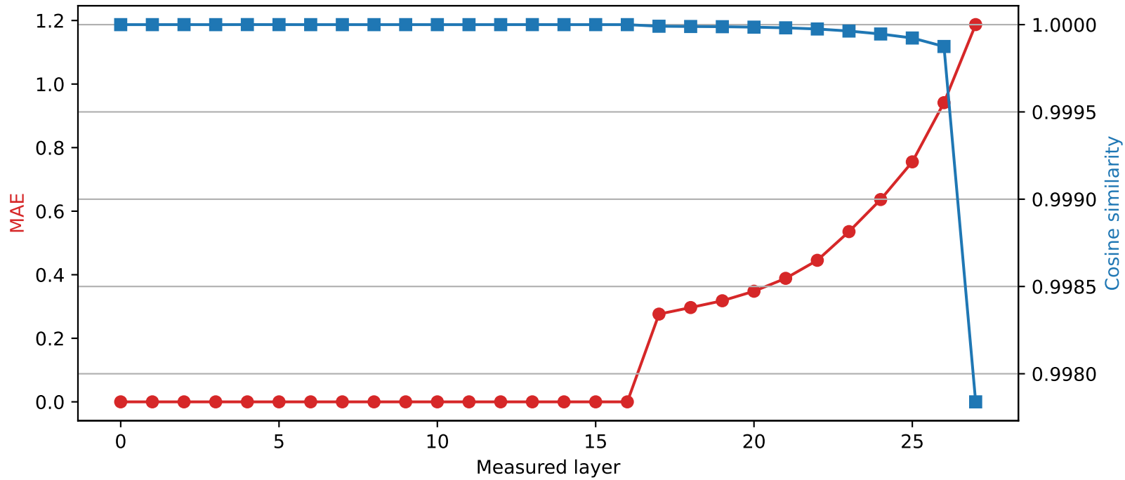
Qwen2.5-7B-Instruct | Quantized layer 16 | float16 \rightarrow int4
