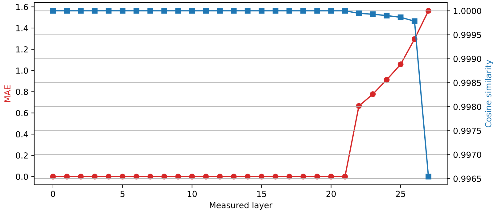
Qwen2.5-7B-Instruct | Quantized layer 21 | float16 \rightarrow int4
