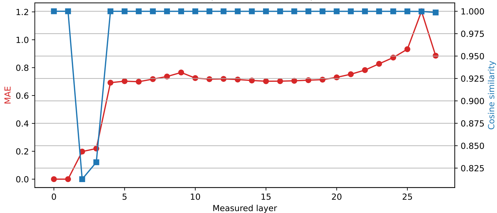
Qwen2.5-7B-Instruct | Quantized layer 1 | float16 \rightarrow int4
