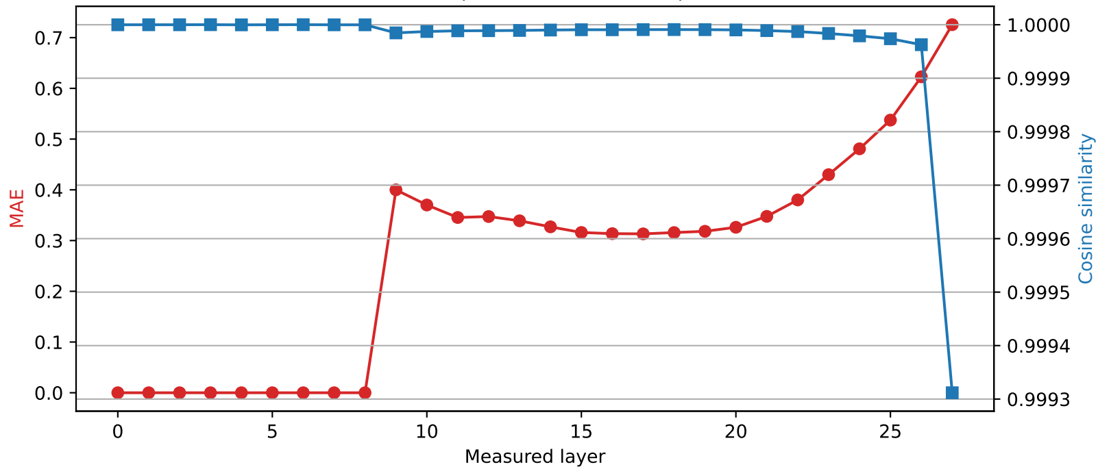
Qwen2.5-7B-Instruct | Quantized layer 8 | float16 → int4
