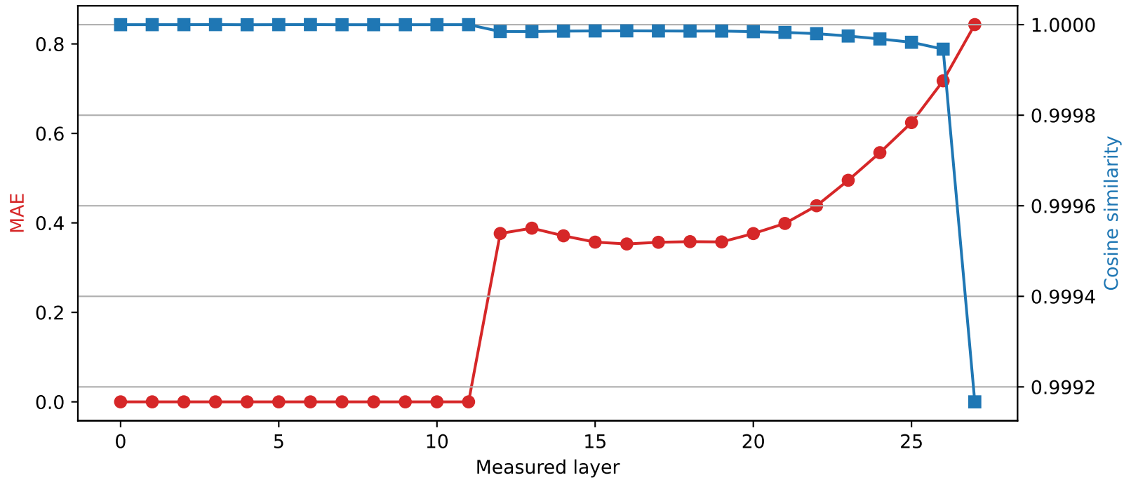
Qwen2.5-7B-Instruct | Quantized layer 11 | float16 \rightarrow int4
